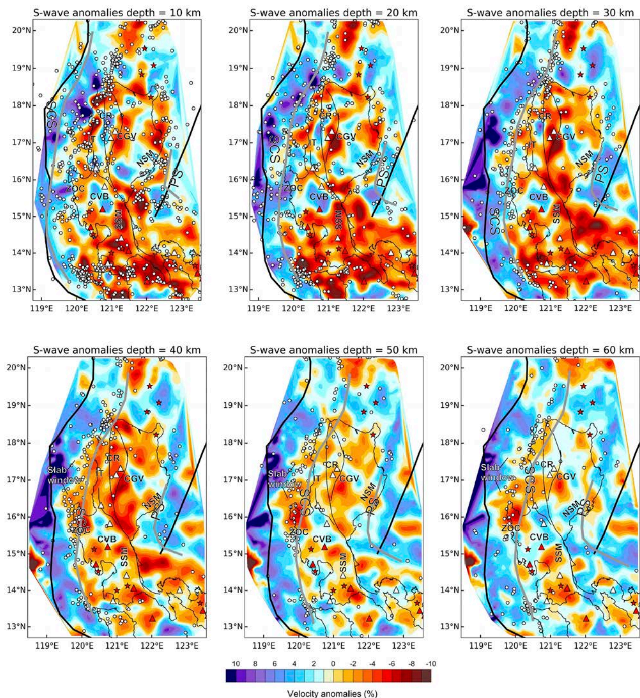
FIGURE 10 Map view of S-wave tomography of different depths. The symbols and abbreviations are the same as those in Figure 9.
