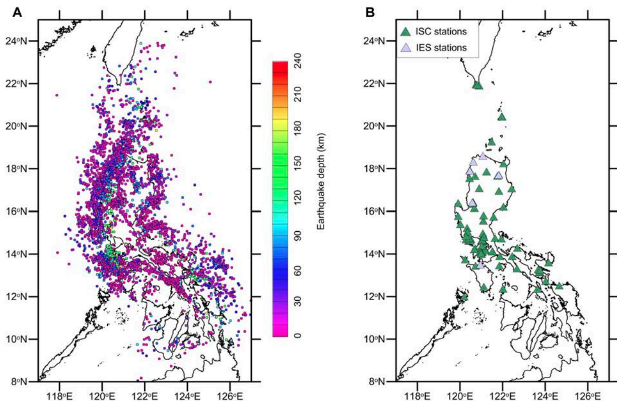
FIGURE 2 Distribution of (A) earthquake events and (B) seismic stations used in this study. The green triangles indicate stations in the ISC catalog, purple triangles indicate stations of the PHIVOLCS-IES network, and circles indicate earthquakes with colors indicating depth.
